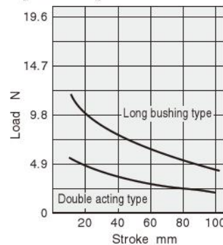
\phi 20 [0.787in.]
