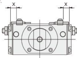
Mounting location of sensor switch for specified angle detection: X
