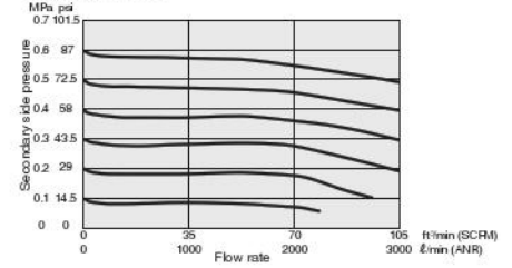
RZ50-F11-03
