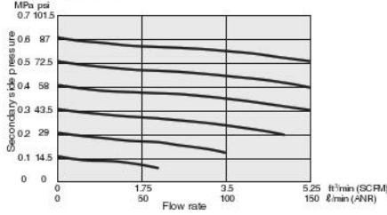
RZ30-F11-01
