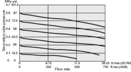
RZ30-F11-02
