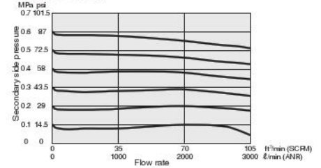
RZ50-F11-04
