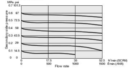
RZ50-F11-02
