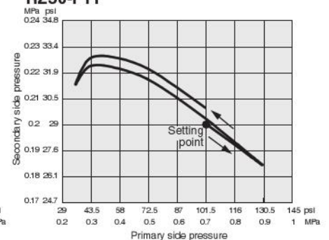
RZ50-F11
