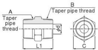
Nipple
