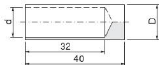
Block off tube
