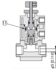
Double acting type: -D
