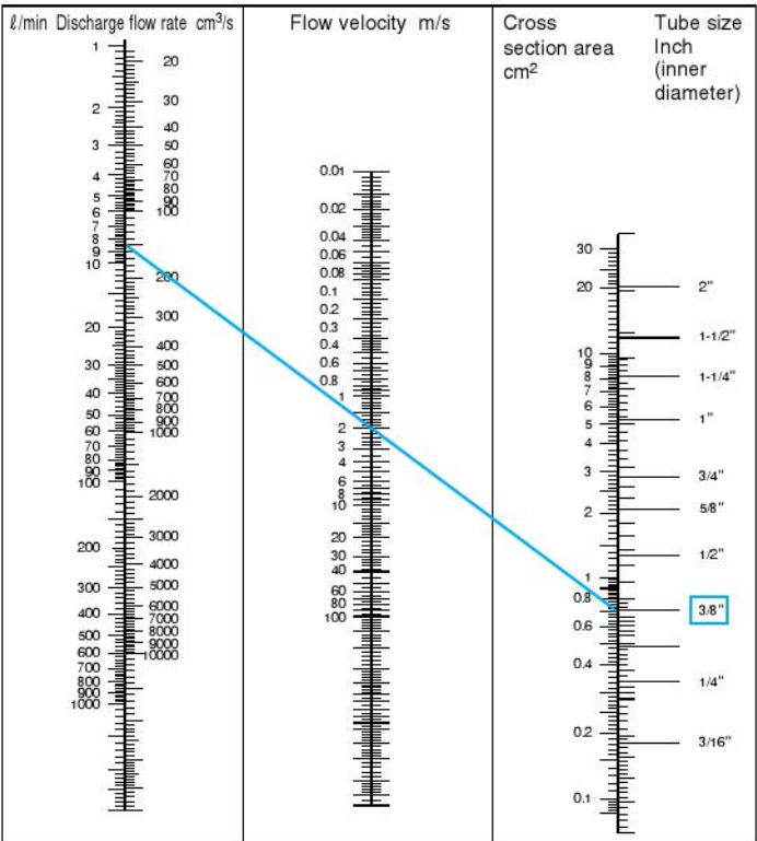
Nomograph
