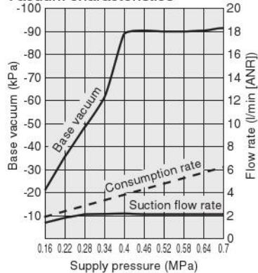
Vacuum characteristics
