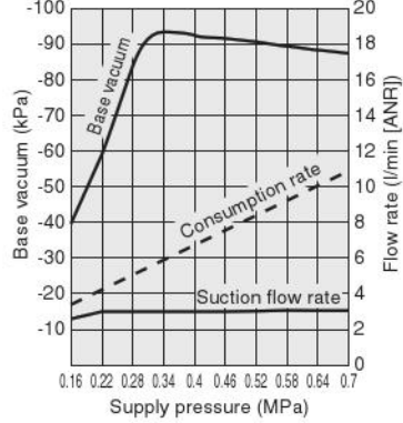
Vacuum characteristics
