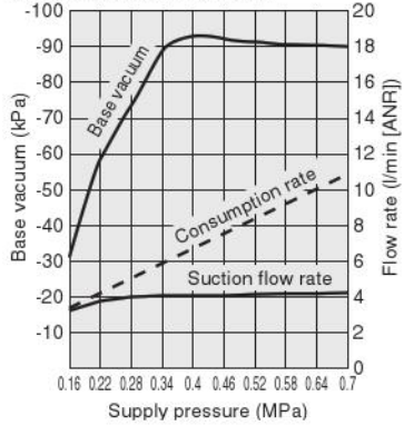
Vacuum characteristics
