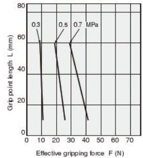
NHBRP-25
