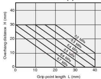
NHBDPG(J)-10 NHBRPG(J)-10
