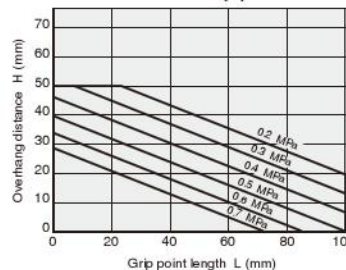
NHBDPG(J)-20 NHBRPG(J)-20
