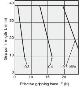
NHBRP-20
