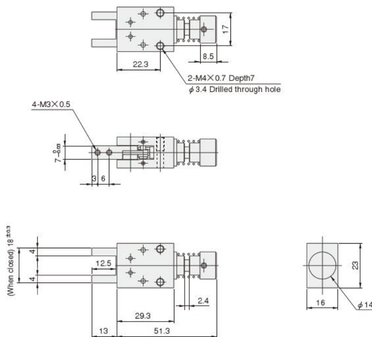
NHBMP-10 (Single acting normally closed type)
