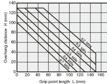
NHBDPG-32
