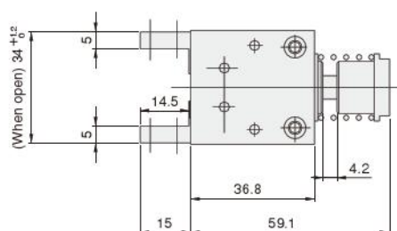
NHBMRP-16 (Single acting normally open type)
