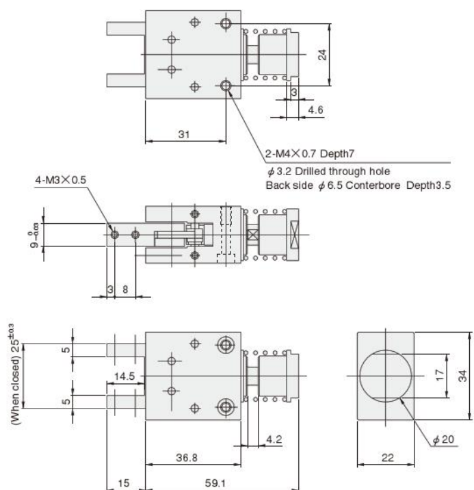
NHBMP-16 (Single acting normally closed type)
