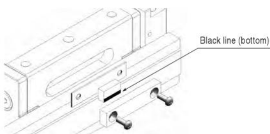
Sensor magnet mounting orientation
