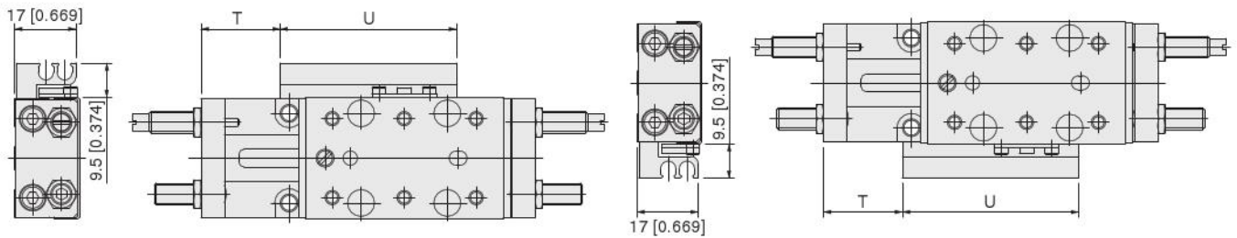
When magnet and sensor rail installed (Piping direction-R)
