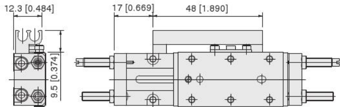
When magnet and sensor rail installed (Piping direction-R)
