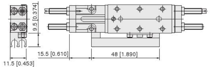
When magnet and sensor rail installed (Piping direction-L)
