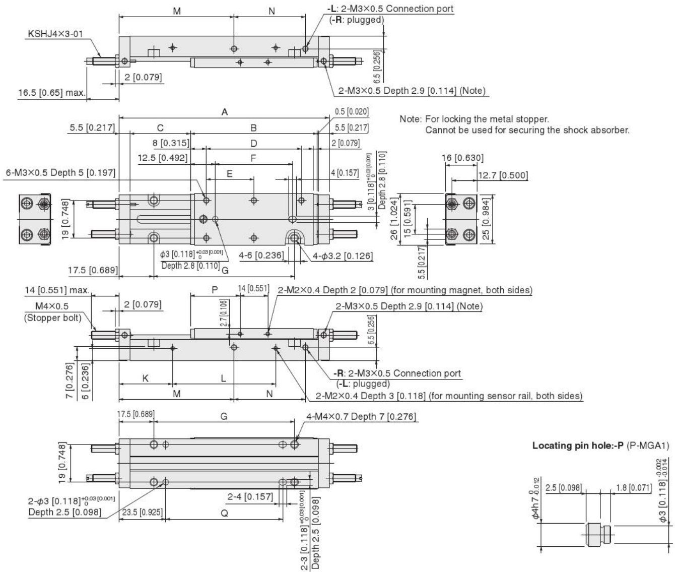
When magnet and sensor rail installed (Piping direction-R)
