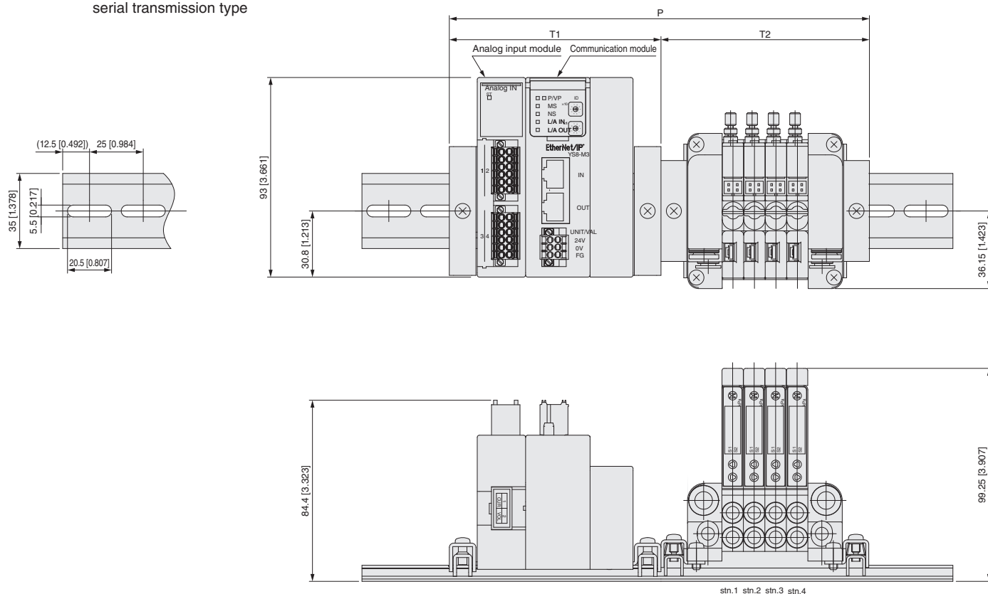
Dimension table for A1
