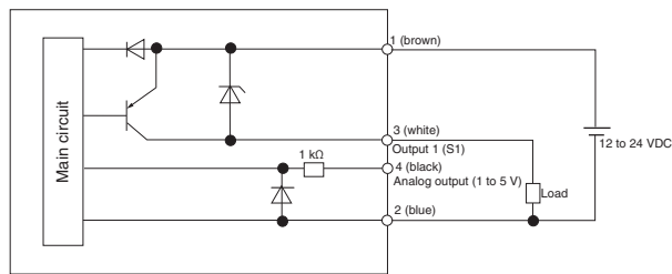
LSMEZ-PDA (PNP, 1-output/analog output type)
