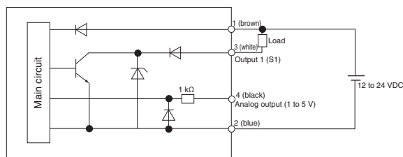
LSMEZ-NDA (NPN, 1-output/analog output type)
