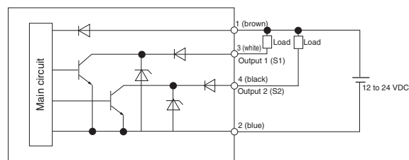
LSMEZ-ND2 (NPN, 2-output type)
