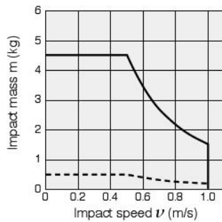
● KSHP8 × 6 (-F11)
