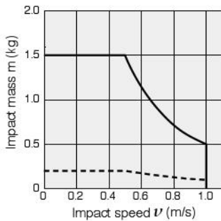
● KSHP6 × 4 (-F11)
