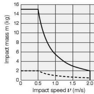
● KSHP12 × 10 (-F11)
