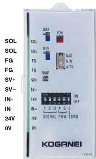
Proportional control valve controller KFPC1
