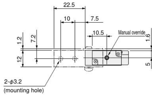
L-type plug connector
