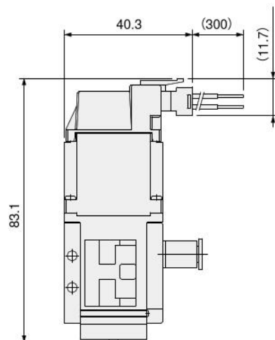
L-type plug connector
