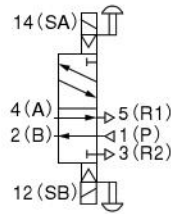
JE12F6 [De-energized condition after energizing solenoid 12 (SB)]
