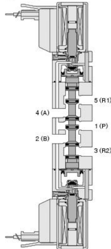
JE12F6 [De-energized condition after energizing solenoid 12 (SB)]
