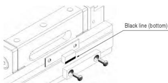
Sensor magnet mounting orientation
