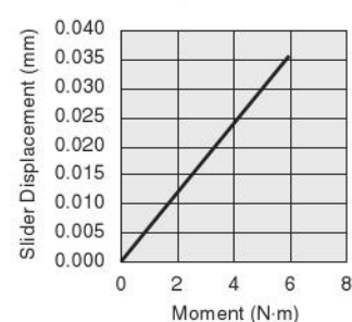
Yawing Moment ( M_y )
