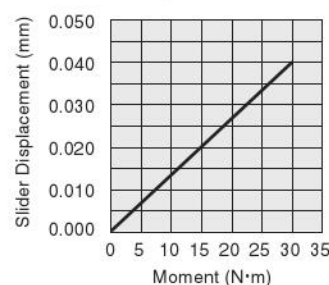
Yawing Moment ( M_y )
