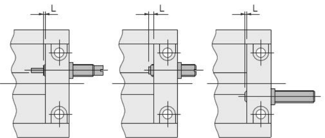
Shock absorber
