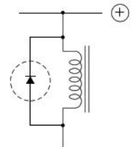
Surge voltage absorption circuit
