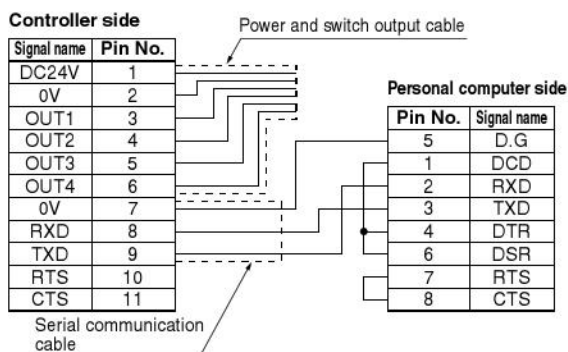
D-sub 9 pin configuration
