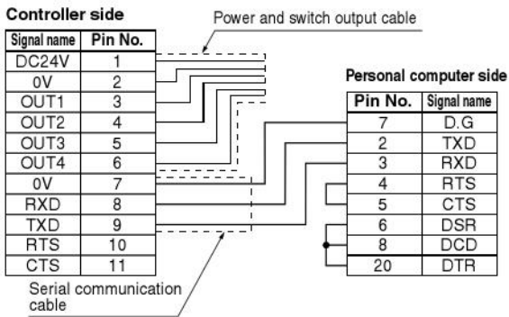
D-sub 25 pin configuration
