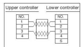
Connector terminal arrangement (Lower controller)
