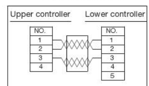
Connector terminal arrangement (Lower controller)
