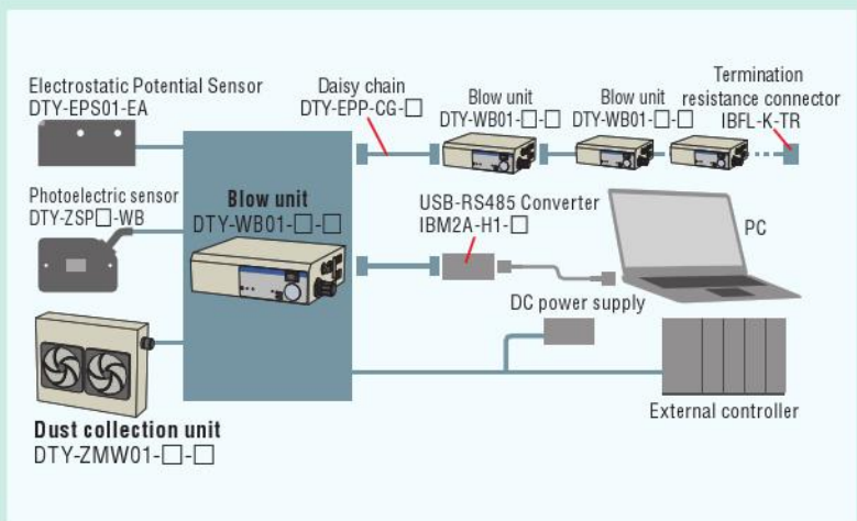
Support Software
