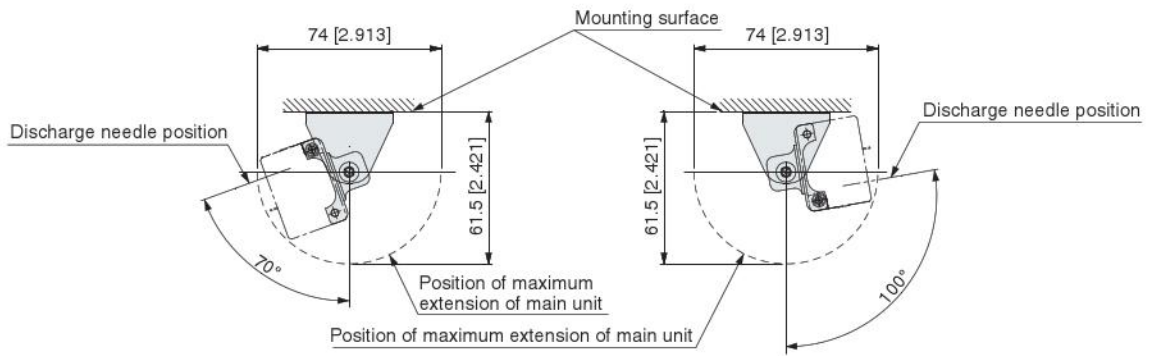
Range of possible installations when mounting DTY-BX01-□-□
