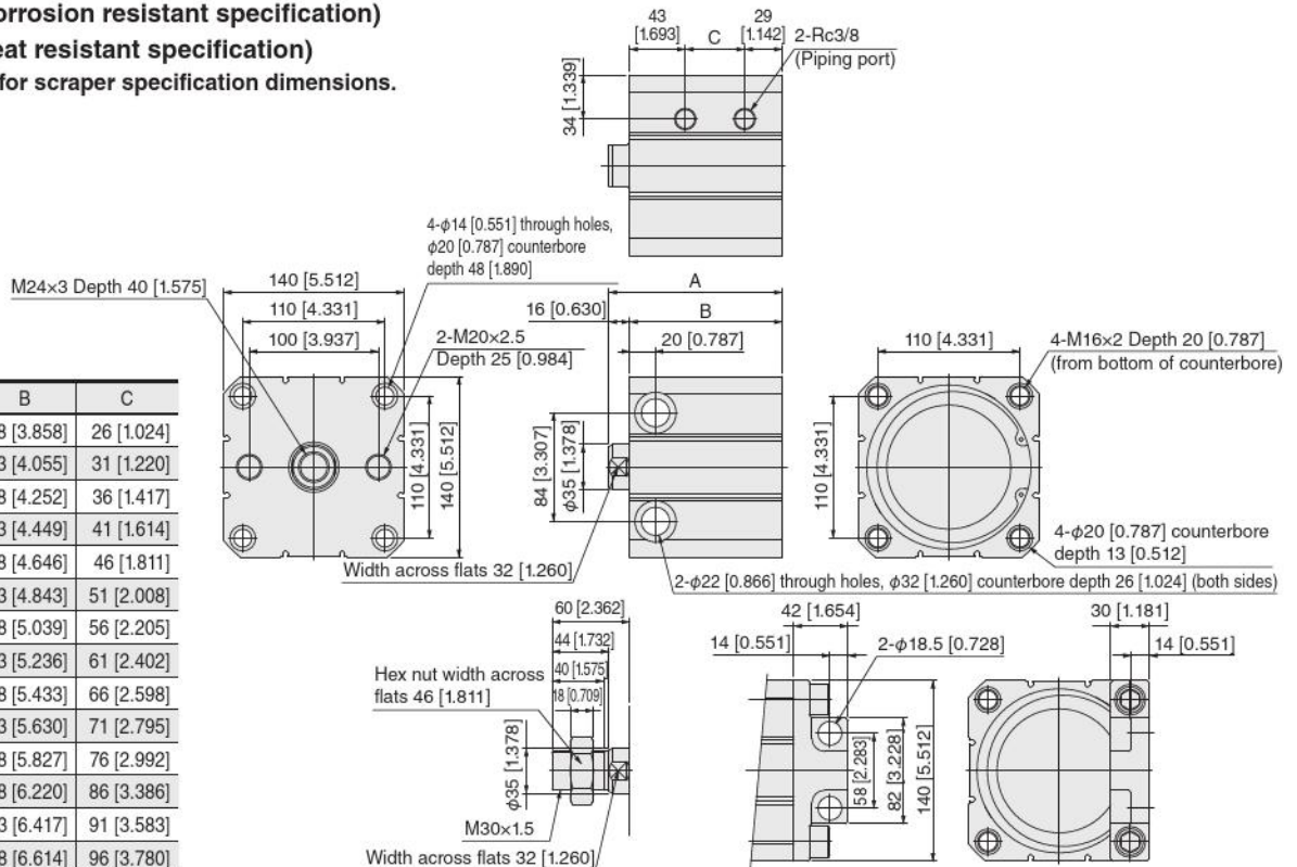
-B: Male thread specifications
