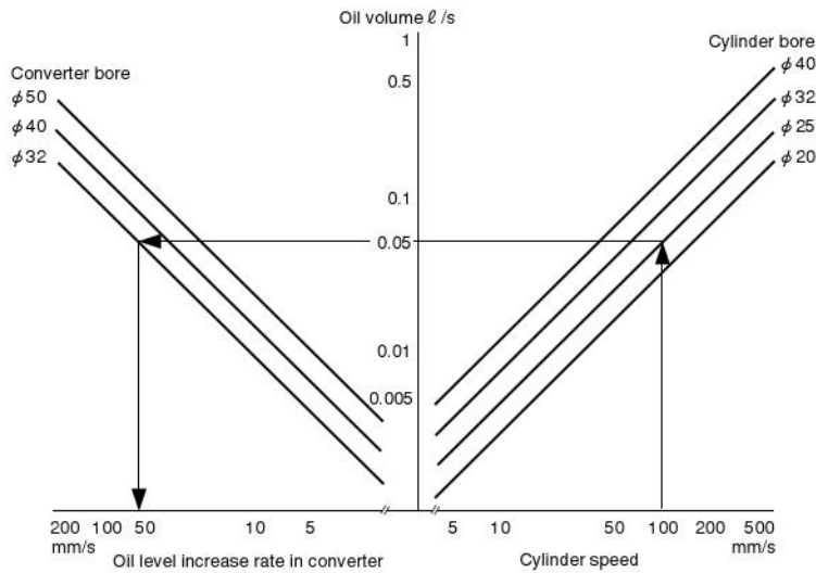
Graph 2: Quick check for converter oil level displacement
