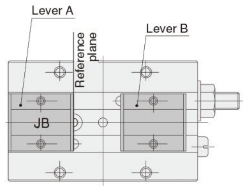
External appearance
