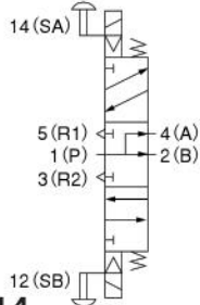
(Both solenoids 14(SA) and 12(SB) are de-energized.)
