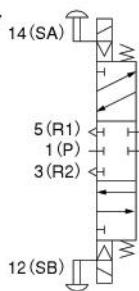
Closed center
