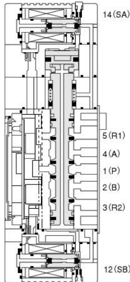
(Both solenoids 14(SA) and 12(SB) are de-energized.)
