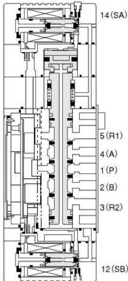
(Both solenoids 14(SA) and 12(SB) are de-energized.)
