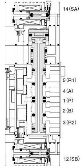
(Both solenoids 14(SA) and 12(SB) are de-energized.)
