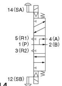
Pressure center
