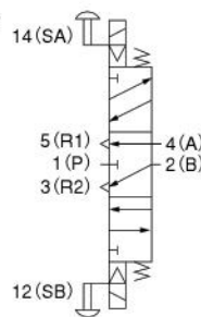
Exhaust center
