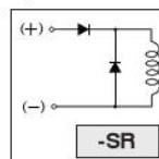
Flywheel diode
