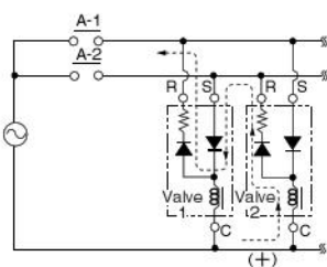
Incorrect wiring
